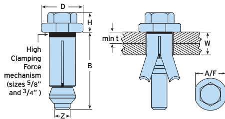
a) Hexagonal
