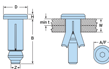
b) Countersunk
