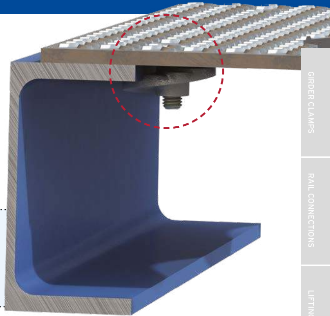
Position of hole centers: \frac{1}{2} flange width - \frac{1}{2} A + \frac{9}{16} inch
