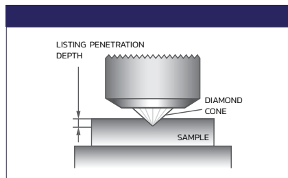
Rockwell Testing
