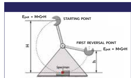
Charpy Testing
